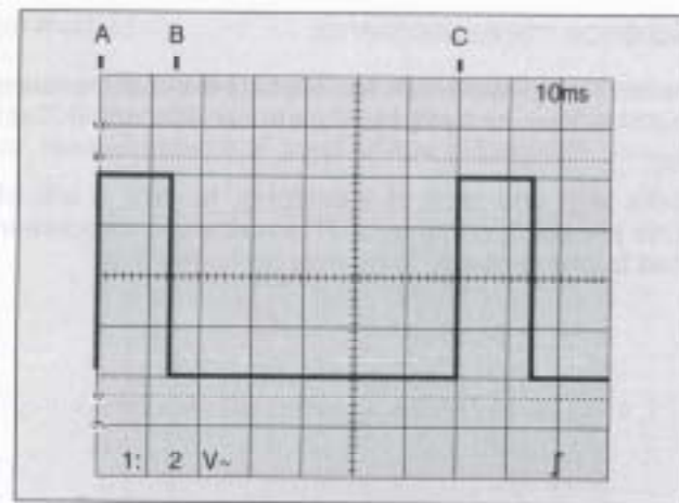
10ms INTERVAL
